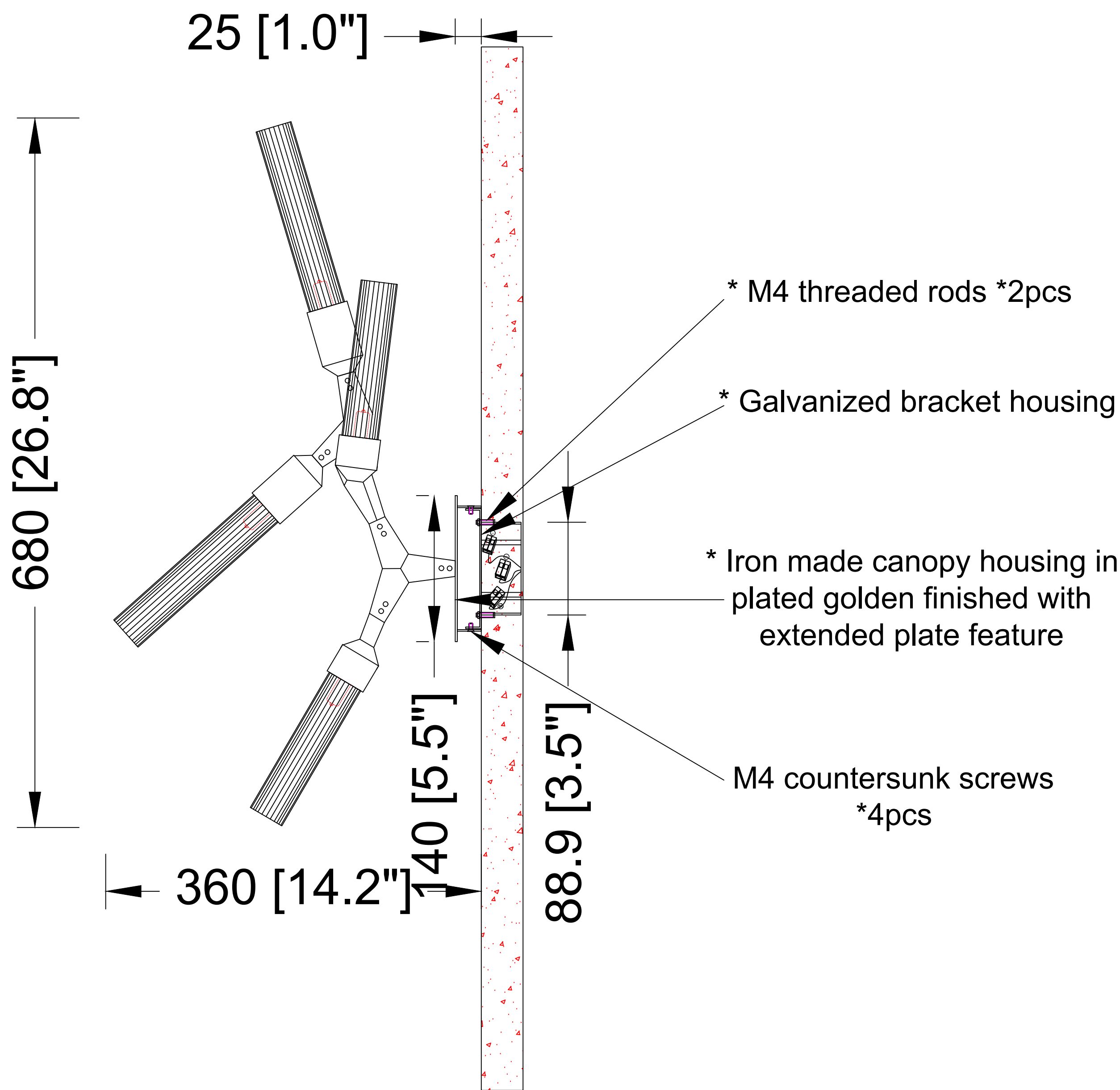
SIDE VIEW
