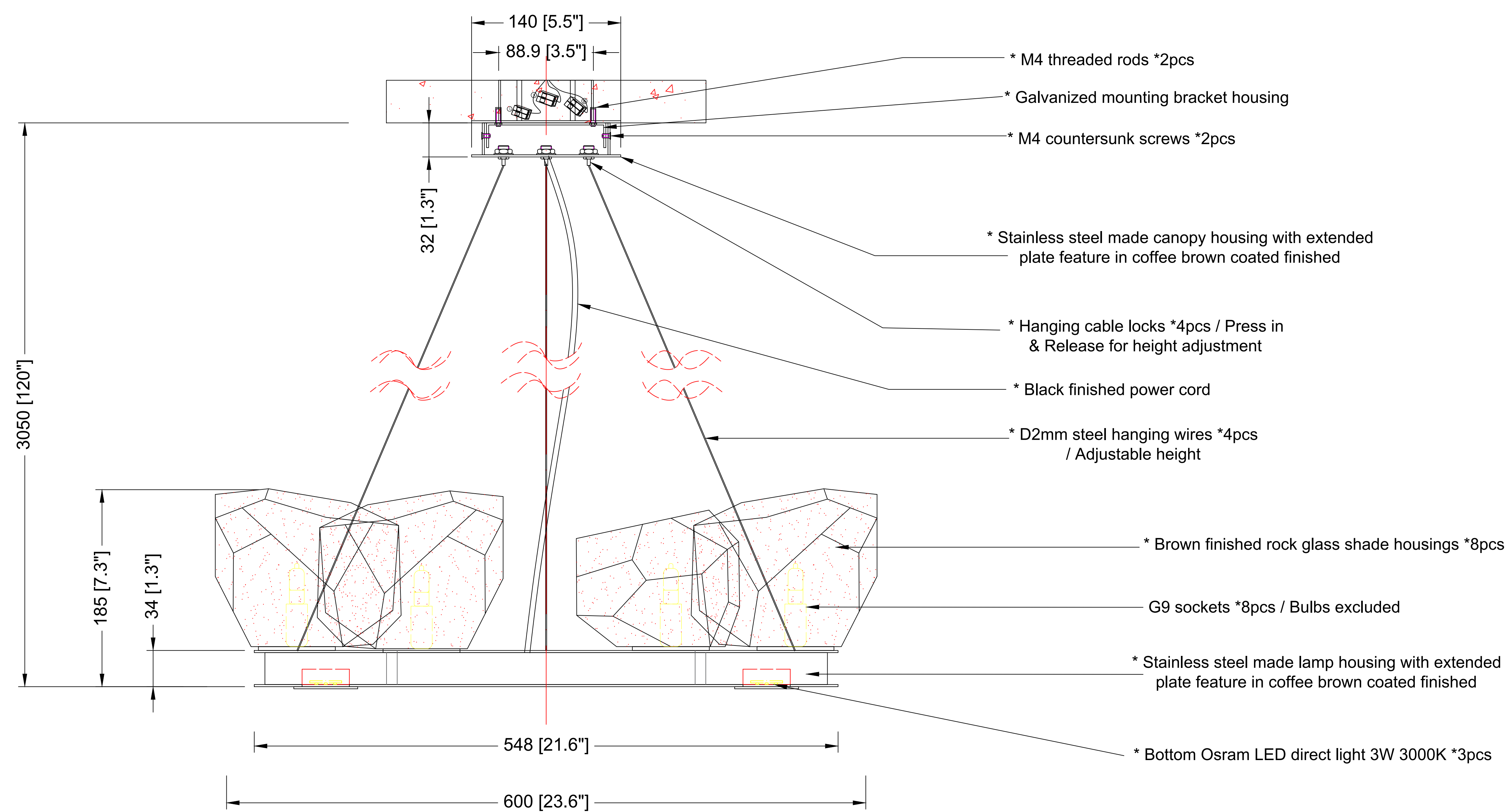
ELEVATION VIEW
