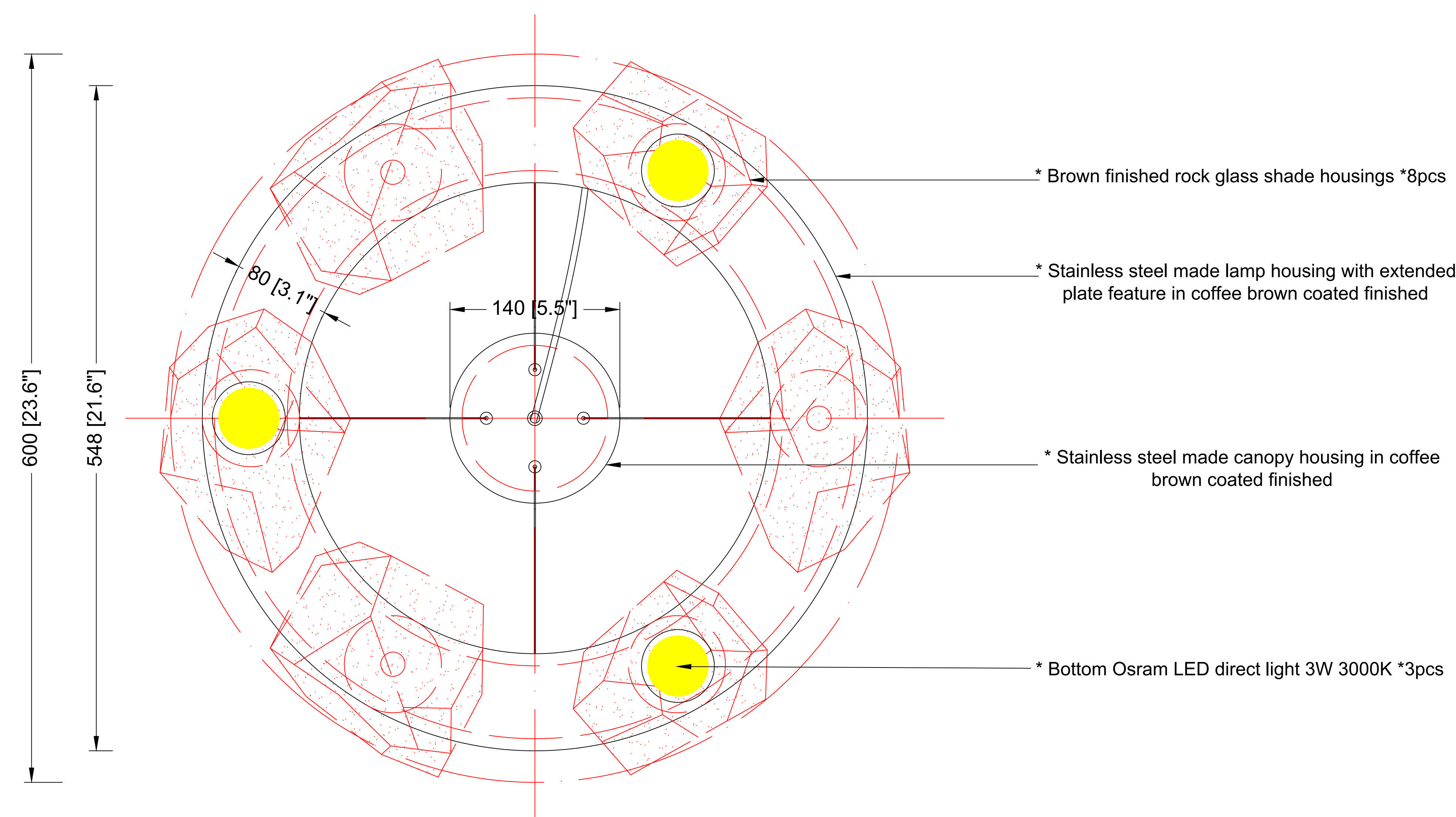
BOTTOM VIEW
