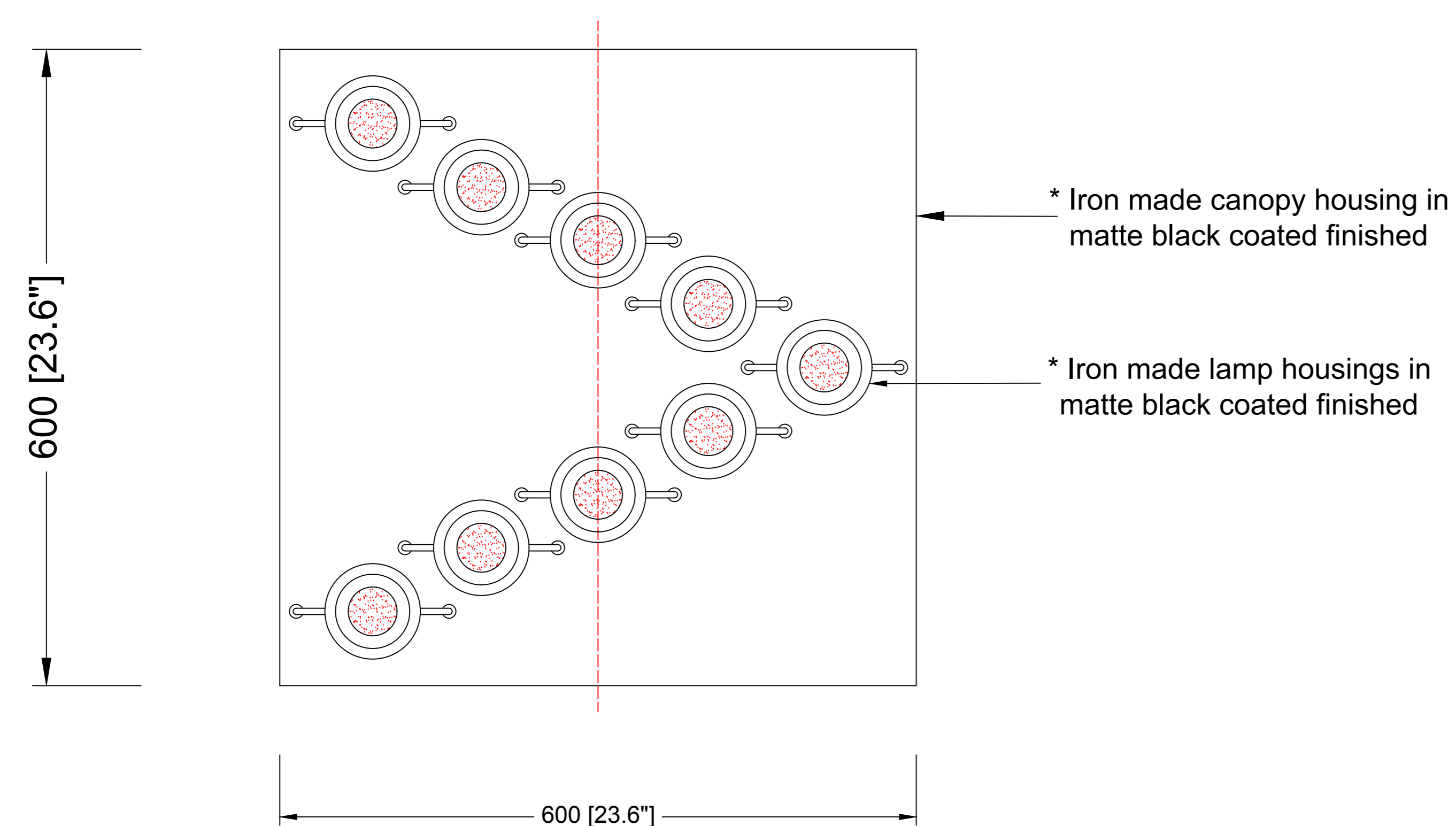
BOTTOM VIEW
