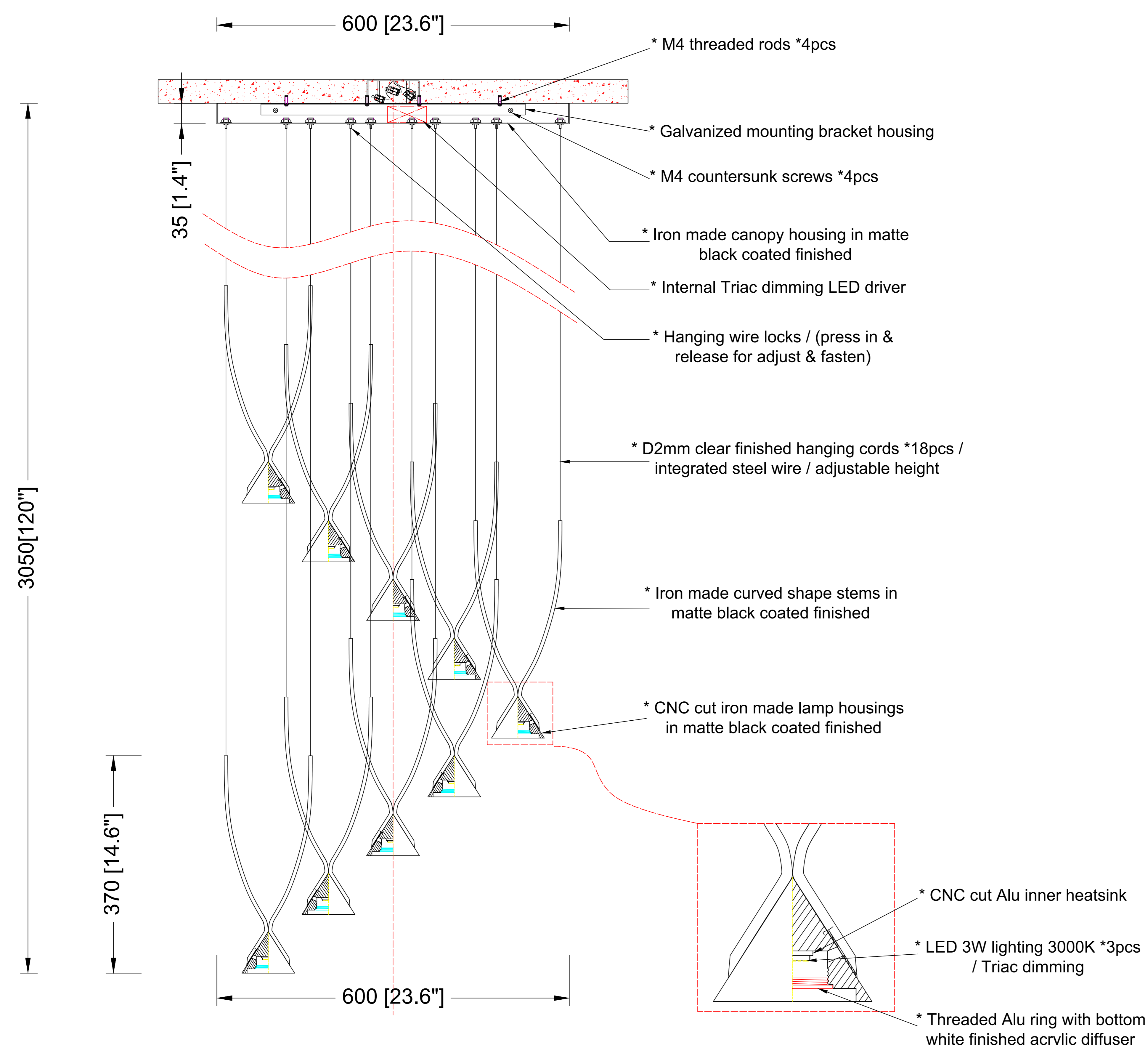
ELEVATION VIEW
