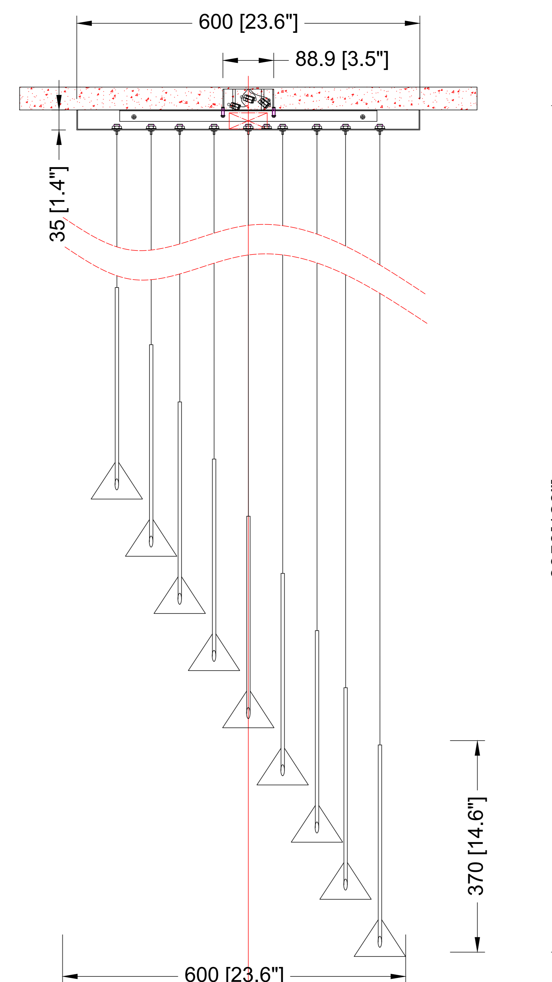
SIDE VIEW
