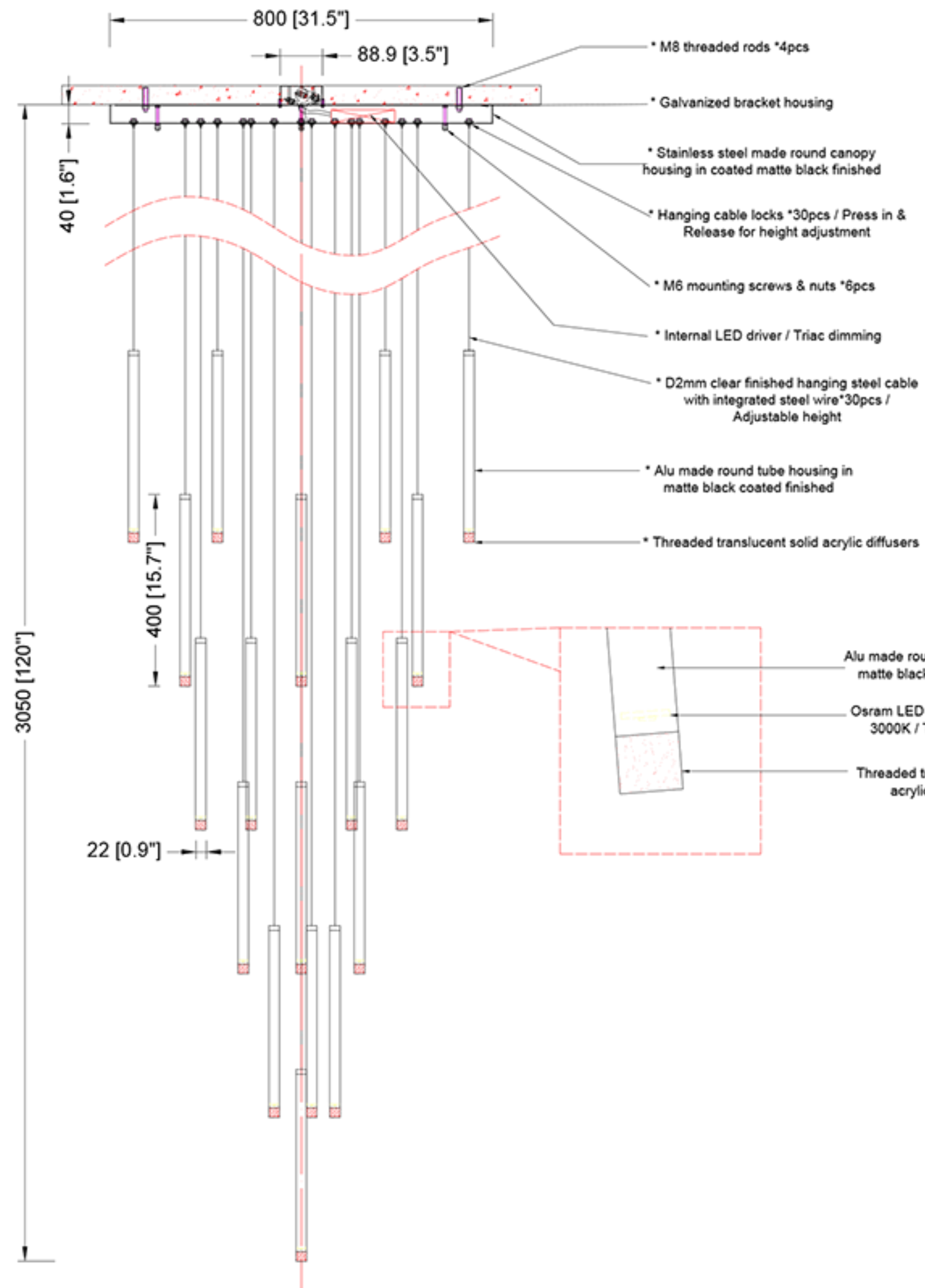
ELEVATION VIEW
