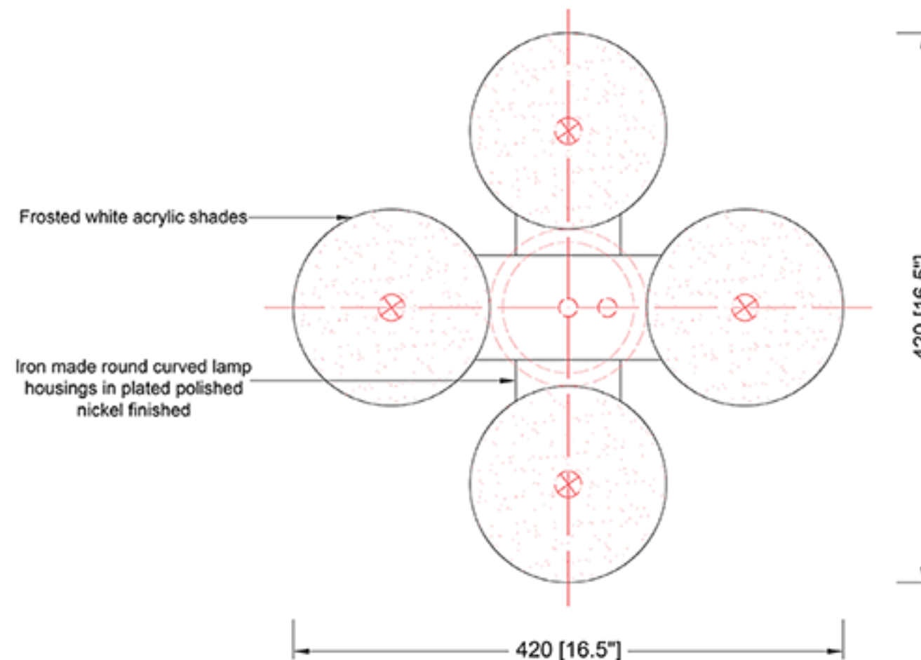
BOTTOM VIEW
